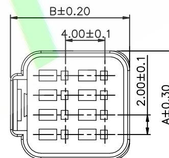
08 PIN DUAL ROW
