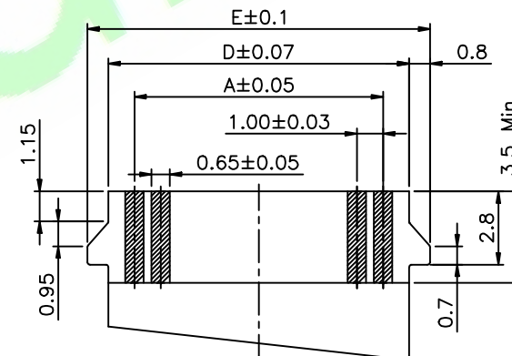
Accommodated FFC/FPC
