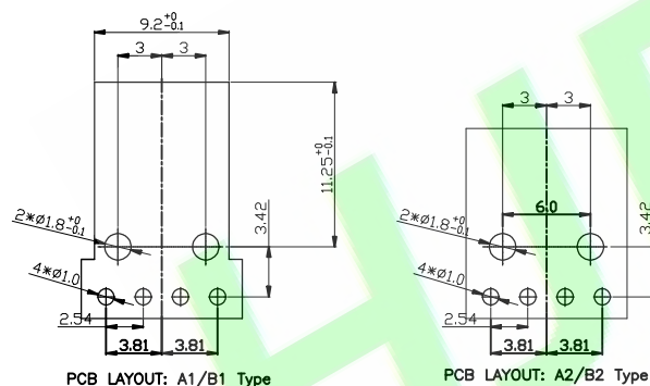
PCB LAYOUT: A1/B1 Type
